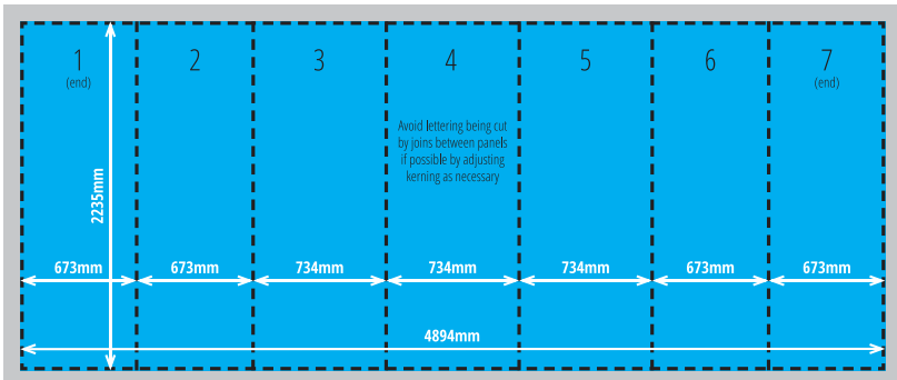
5x3 Hybrid Panel Sizes
