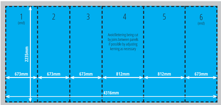
4x3 Hybrid Panel Sizes
