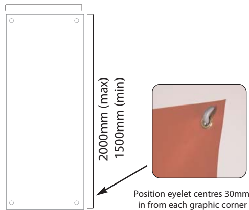
Graphic dimensions and eyelet positioning
